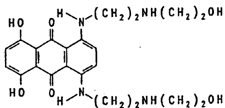
Mitoxantrone
